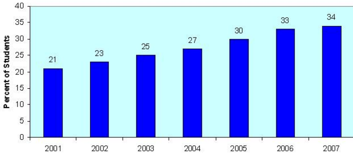
FCAT Scores in Math Percent of Students who are English Language Learners (Grades 3 - 10) Scoring On or Above Grade Level
