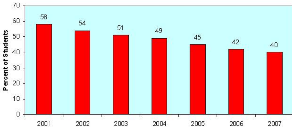
FCAT Scores in Math Percent of Students who are English Language Learners (Grades 3 - 10) Scoring at the Lowest Level
