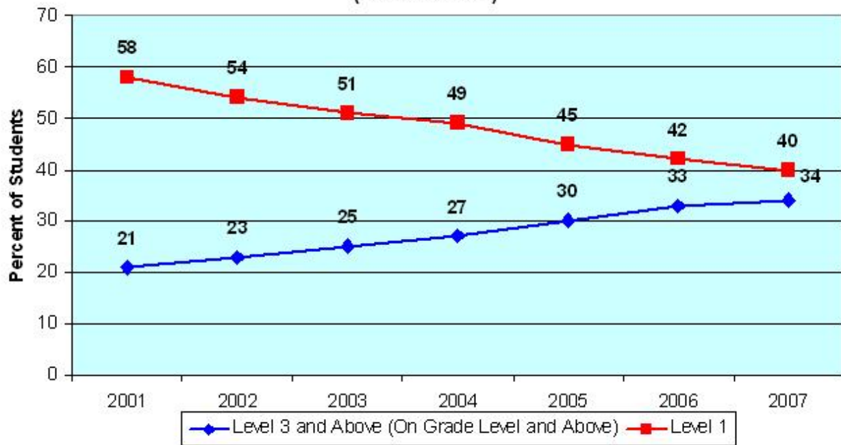
FCAT Scores in Math Percent of Students who are English Language Learners (Grades 3-10)
