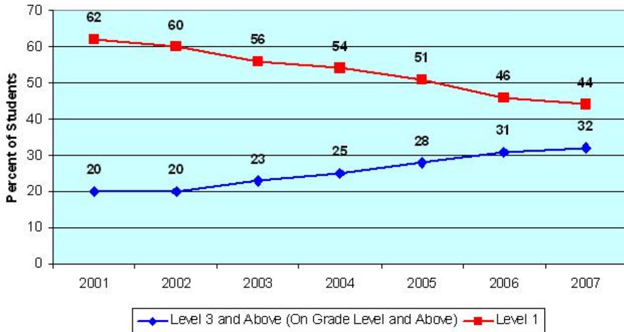
FCAT Scores in Math Percent of Students with Disabilities (Grades 3-10)
